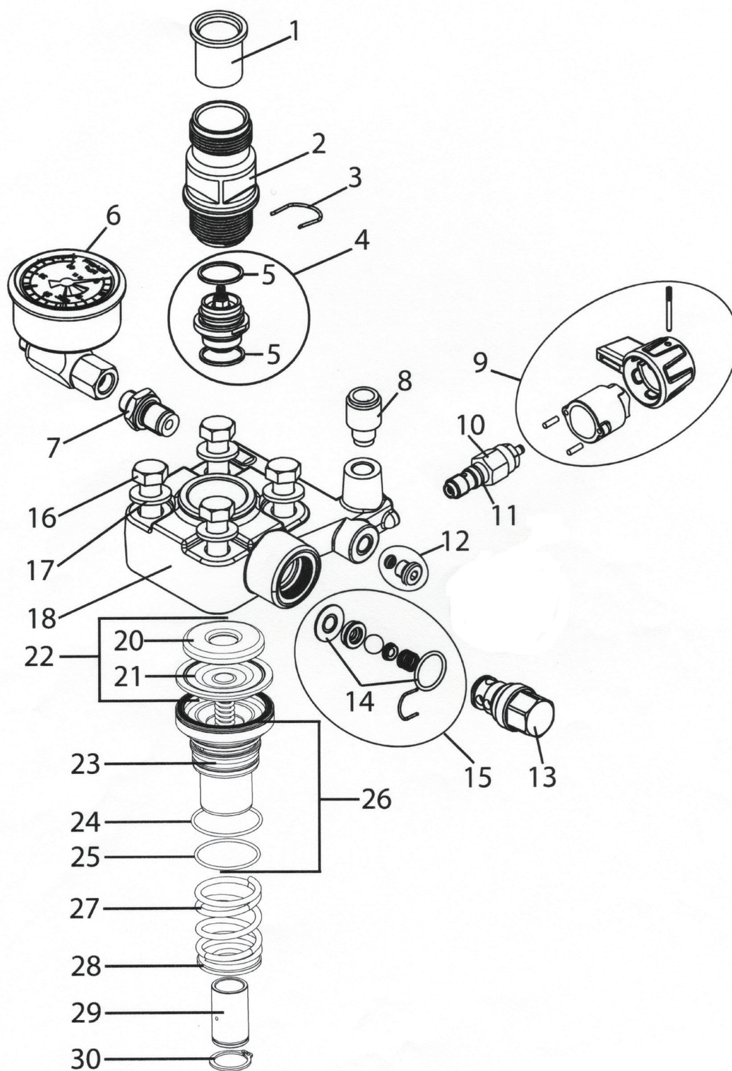
HERO23 pump
